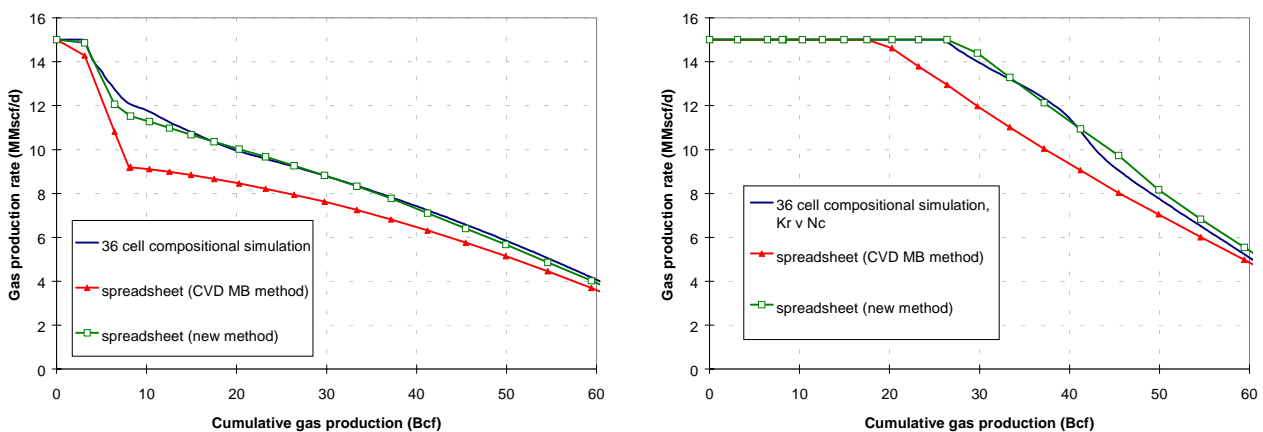
Figure 6. Gas production profiles from spreadsheet and compositional simulation models.
